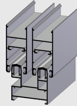
TWO TRACK WITH SLIM INTERLOCK SECTION
