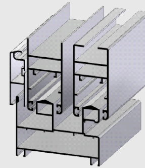
TWO TRACK WITH MOSQUITO SHUTTER OPT.
