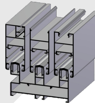
THREE TRACK WITH FLY SCREEN SHUTTER
