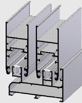
TWO TRACK WITH SLIM INTERLOCK SHUTTER
